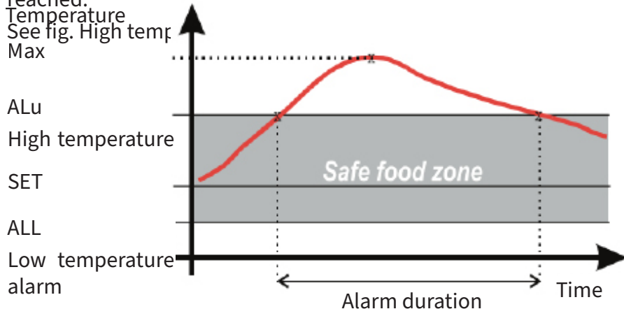
Dixell control panel
